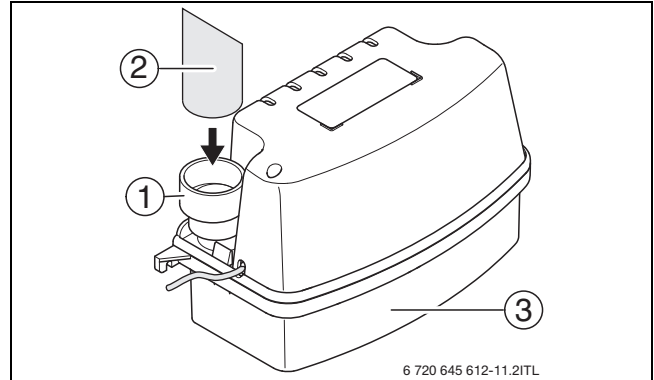
Fig. 7 Fitting the supply hose
