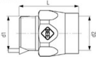
Maßskizze Measured sketch
