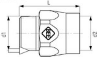
Maßskizze Measured sketch
